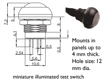
Illustration 2. LED Indicator & Test Switch
