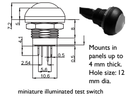
Illustration 2. LED Indicator & Test Switch
