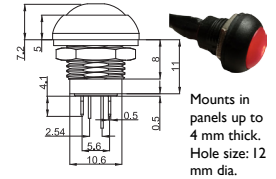
miniature illuminated test switch
