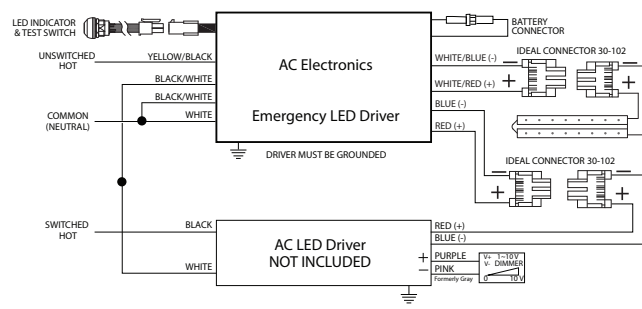
WIRING DIAGRAM FOR SWITCHING THE NEUTRAL WIRE OF THE NORMAL AC LED DRIVER
