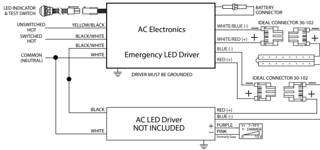
WIRING DIAGRAM FOR SWITCHING THE SWITCHED HOT AC POWER FOR THE NORMAL AC LED DRIVER
