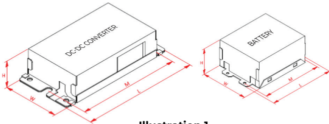
Illustration 1. Unit dimensions, location of Tc, and mounting tabs
